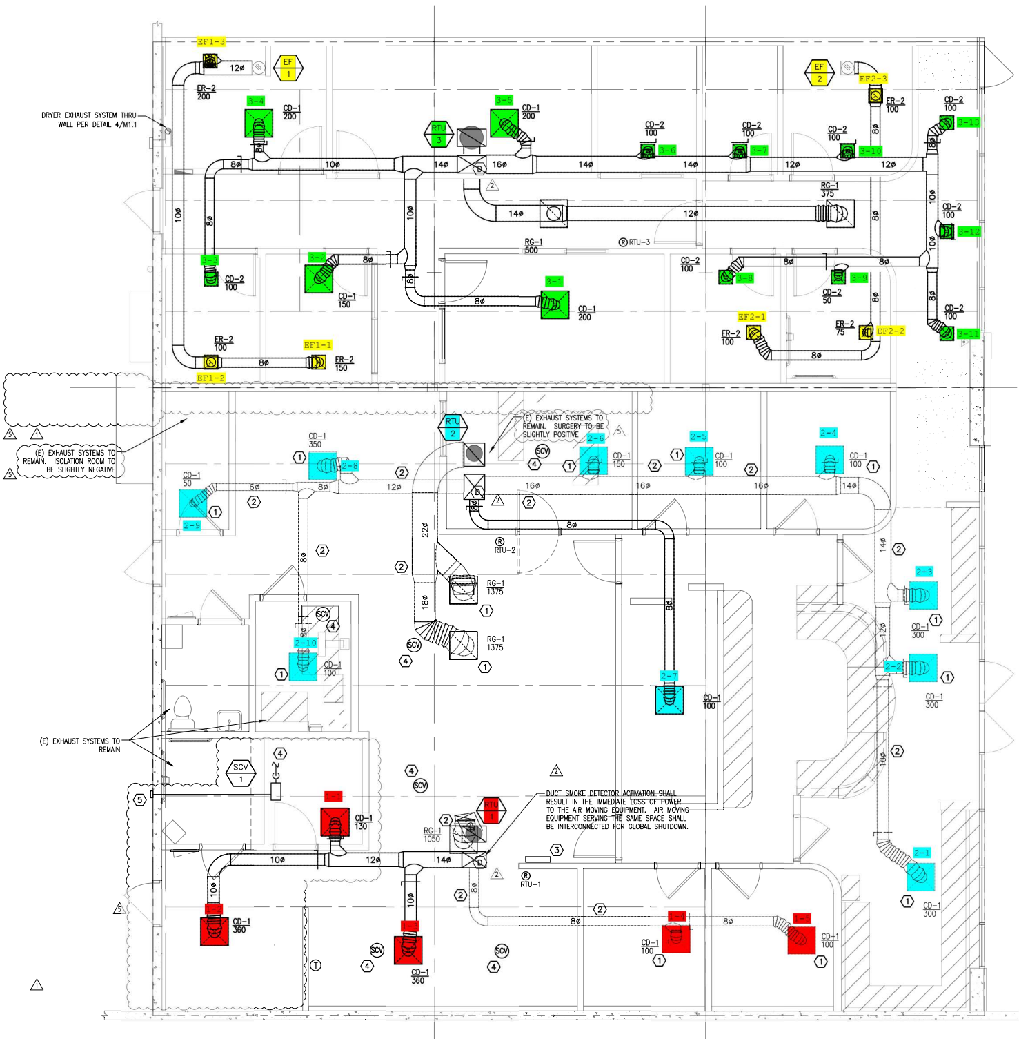
1 MECHANICAL PLAN 1/4" = 1'-0"
